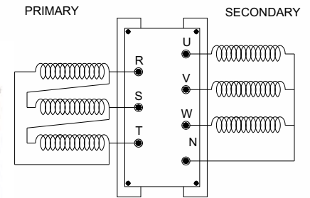
Isolation Transformer Wiring Diagram
