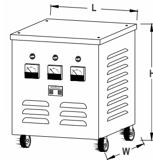
Dimension Drawing
