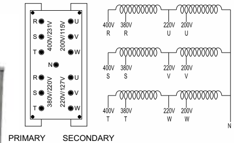
Auto Transformer Wiring Diagram
